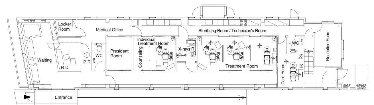
WHITE ESSENCE YOSHIDA DENTAL CLINIC Plan 1: 200
